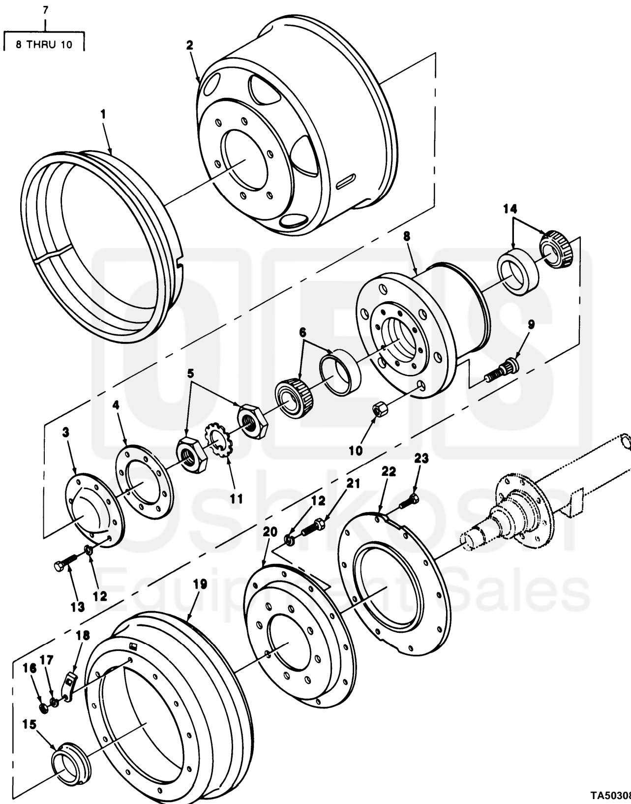
FIGURE 22. HUB AND DRUM ASSEMBLY (M103A1, M105A1, M107A1).
